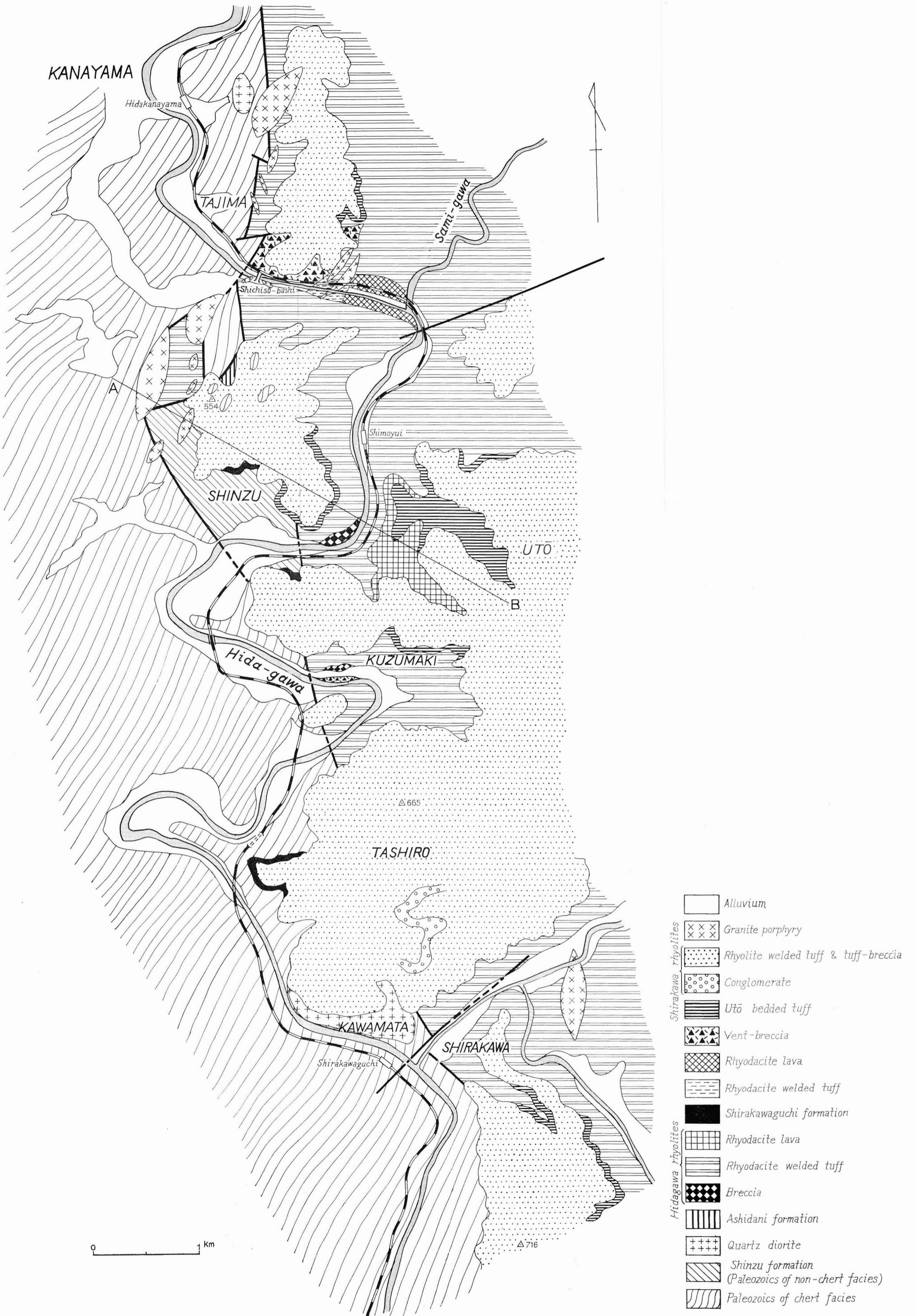
Fig. 5A Geological map of the western margin of the Nōhi rhyolites along the Hida River.
