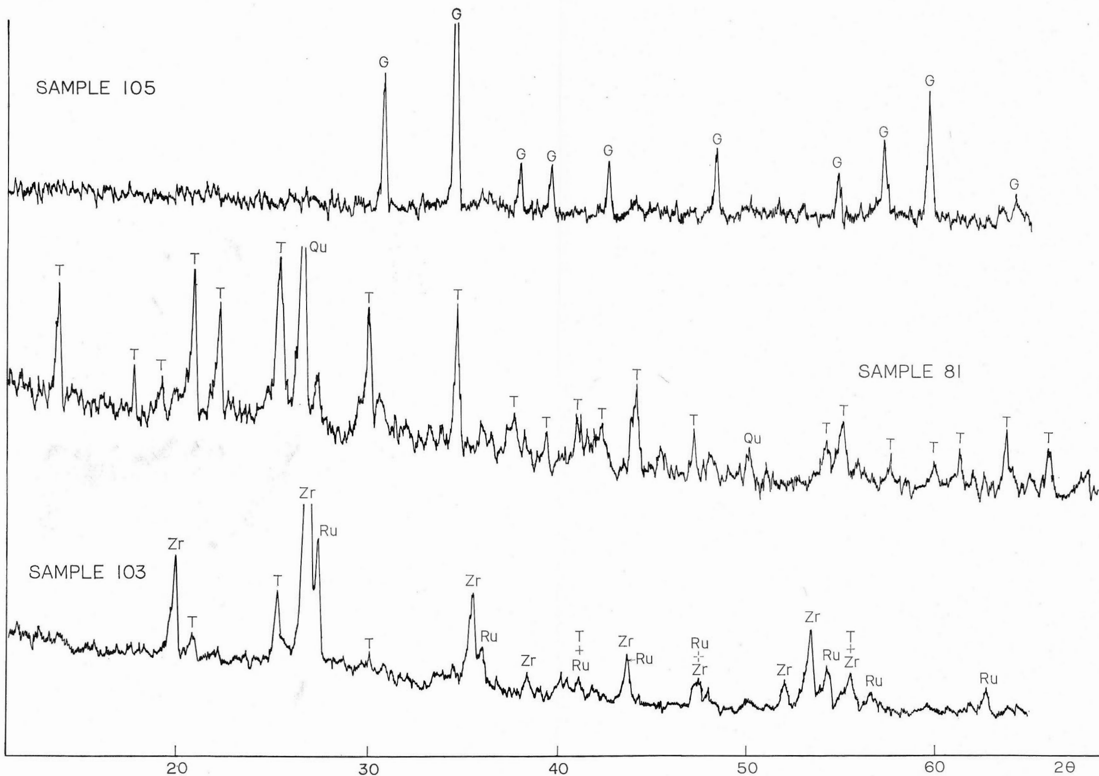
Fig. 3 X-ray diffractometer patterns of samples 105, 81, and 103. G, garnet; Qu, quartz; Ru, rutile; T, tourmaline; Zr, zircon.
