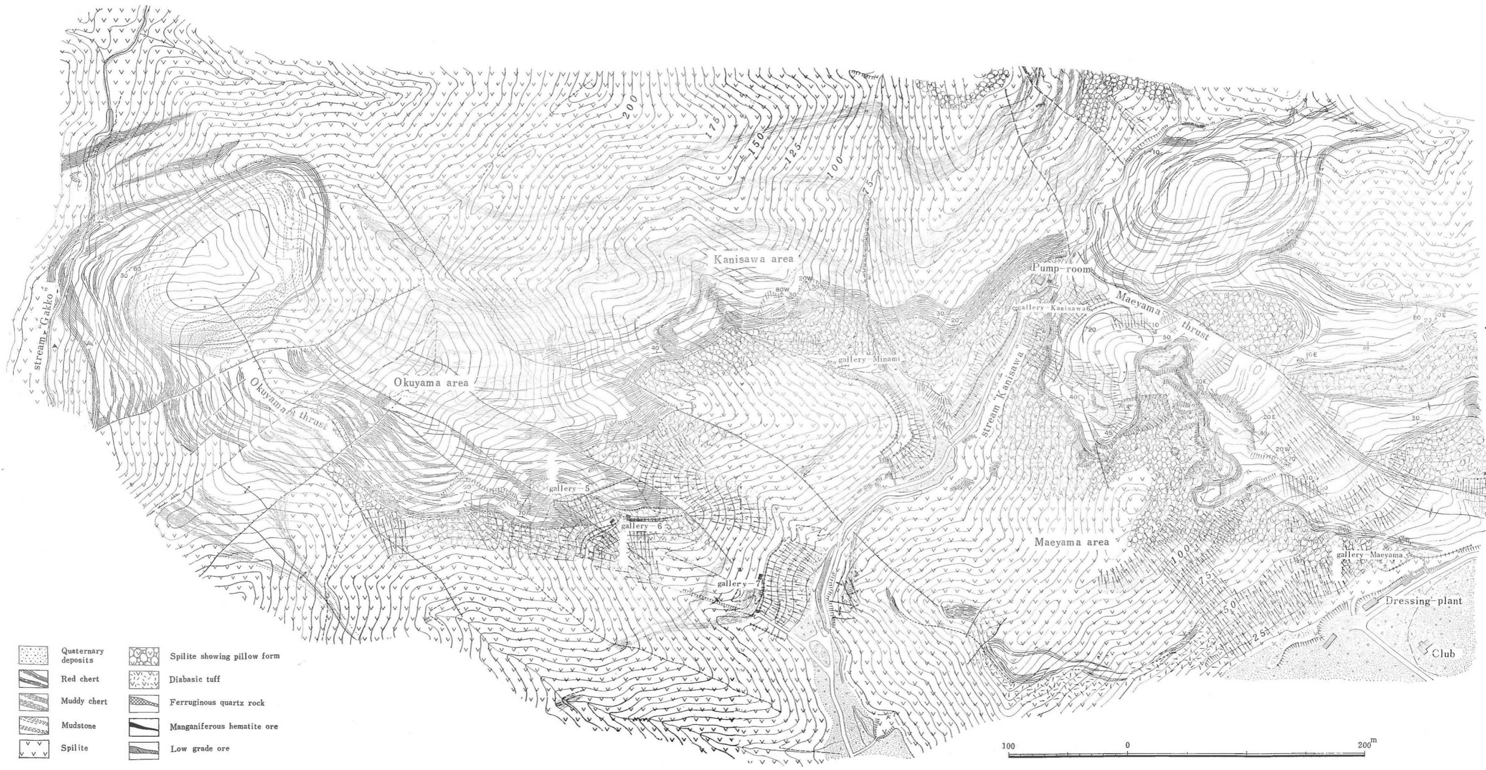
Fig. 7 Geological map of the Tokoro mining area
