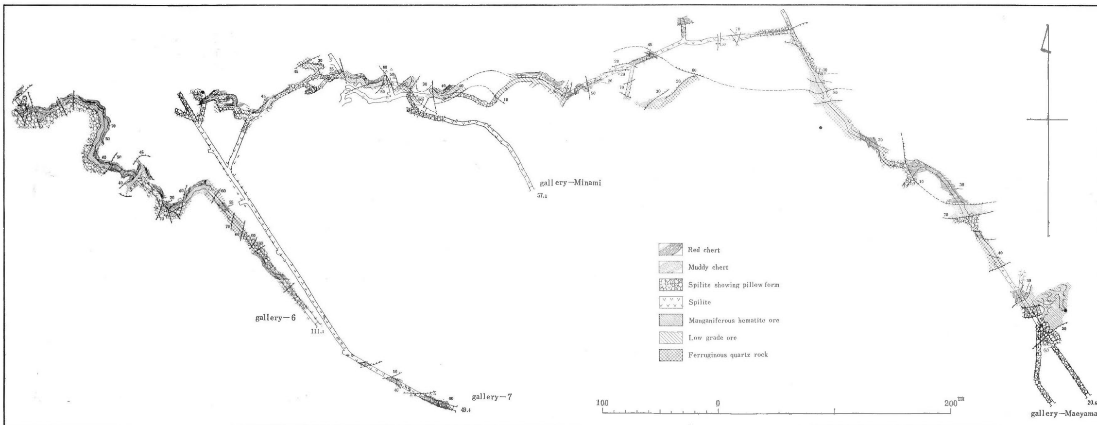
Fig. 8 Underground map of the Tokoro mine
