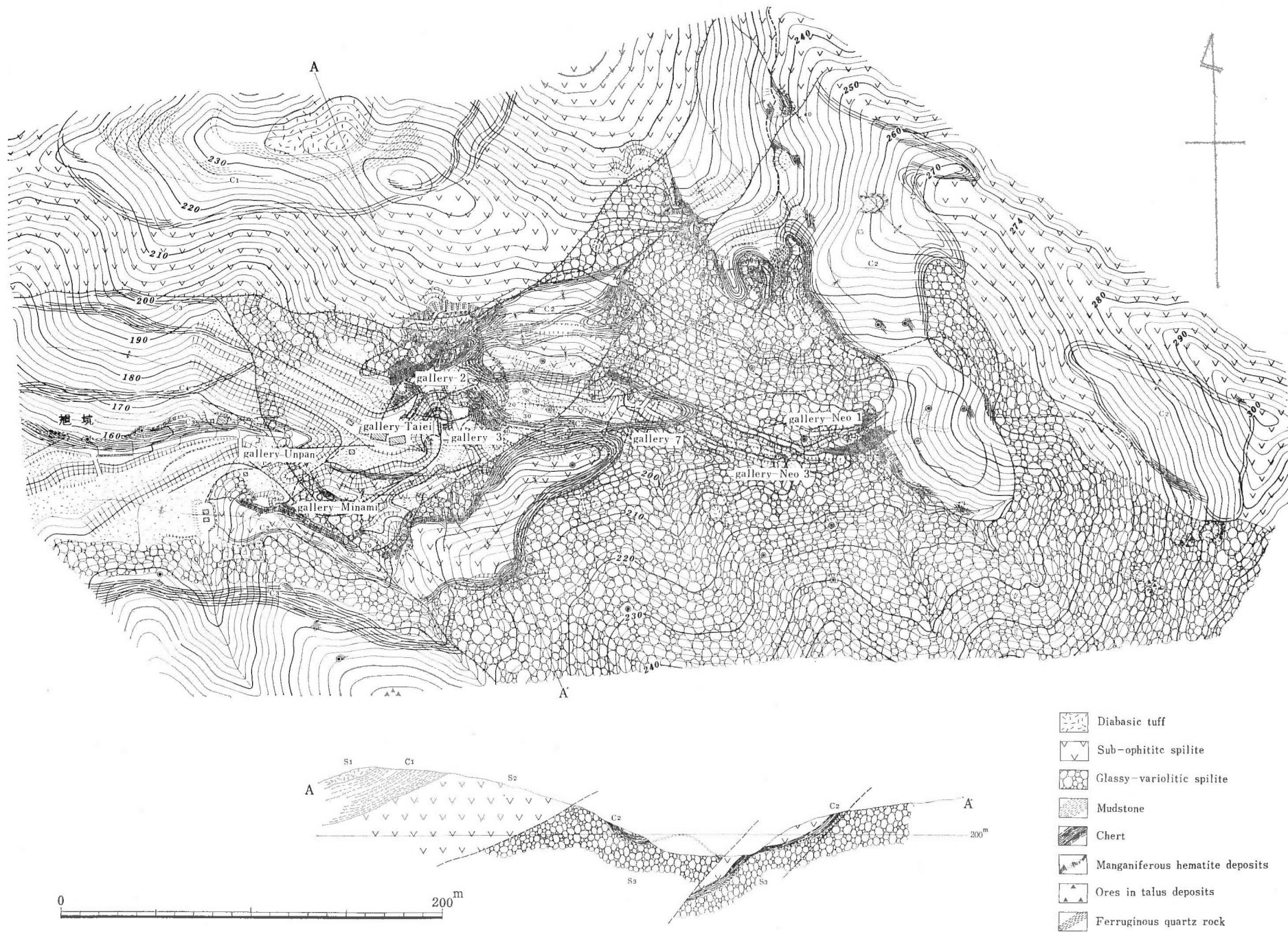
Fig. 9 Geological map of the Nikura mine
