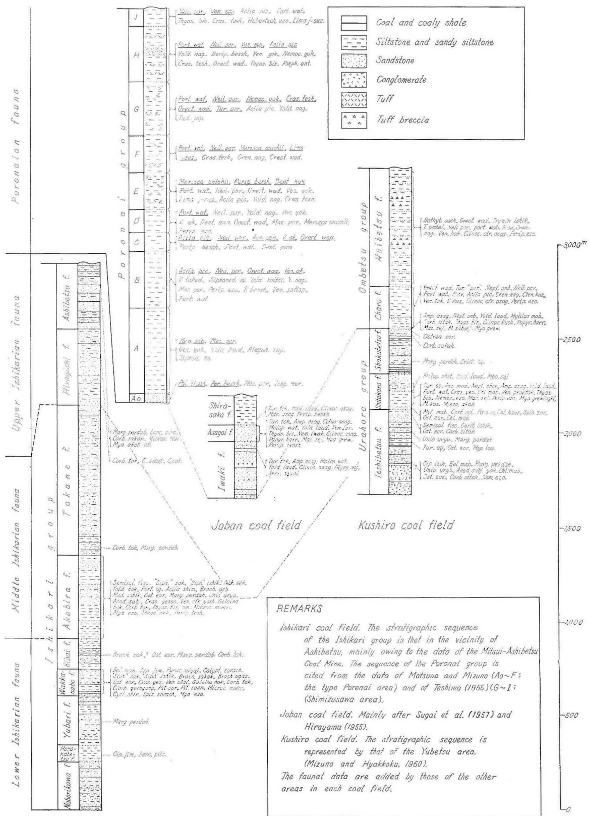
Ishikari coal field
