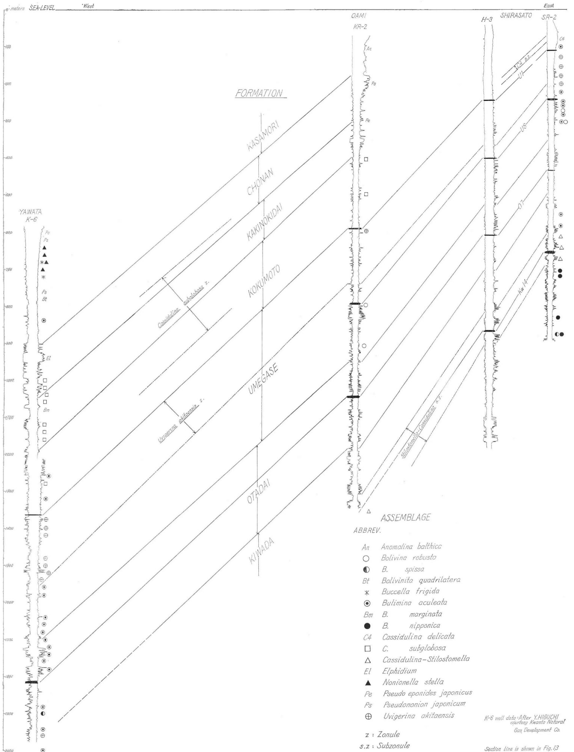
Fig. 14 Correlation between the east and the west coasts of Boso Peninsula.
