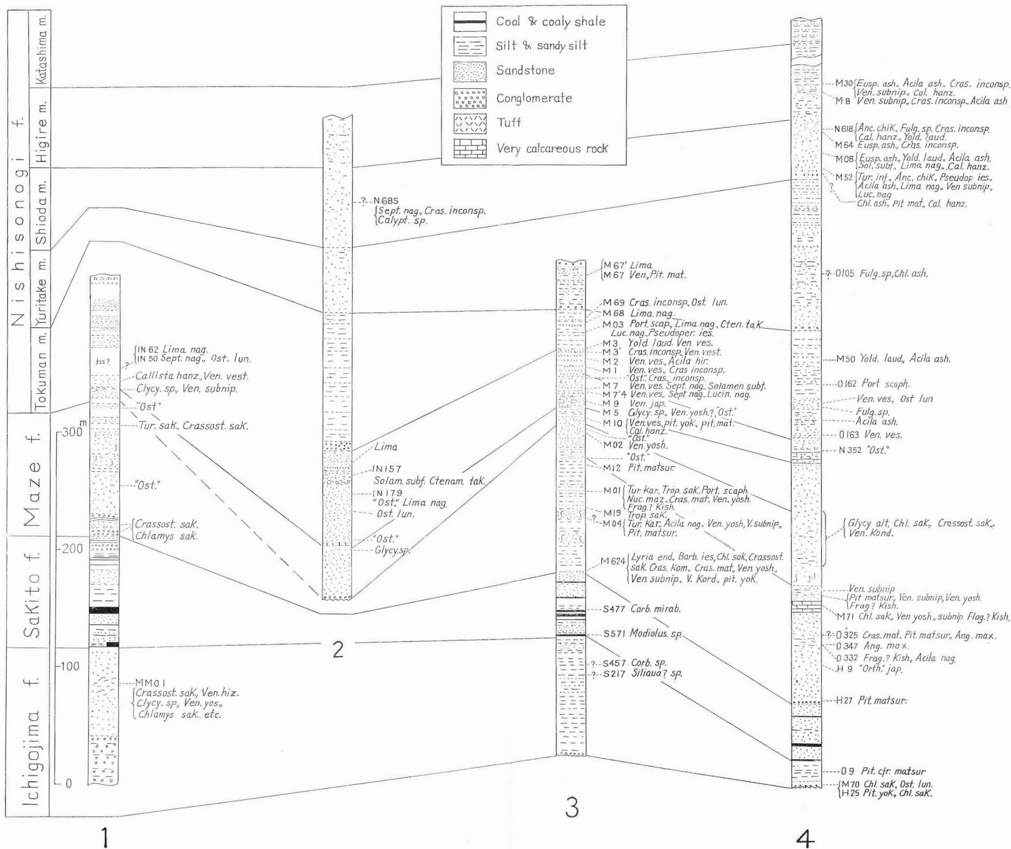
Fig. 11 Columnar sections of the middle and upper Paleogene strata in the Sakito coal field
