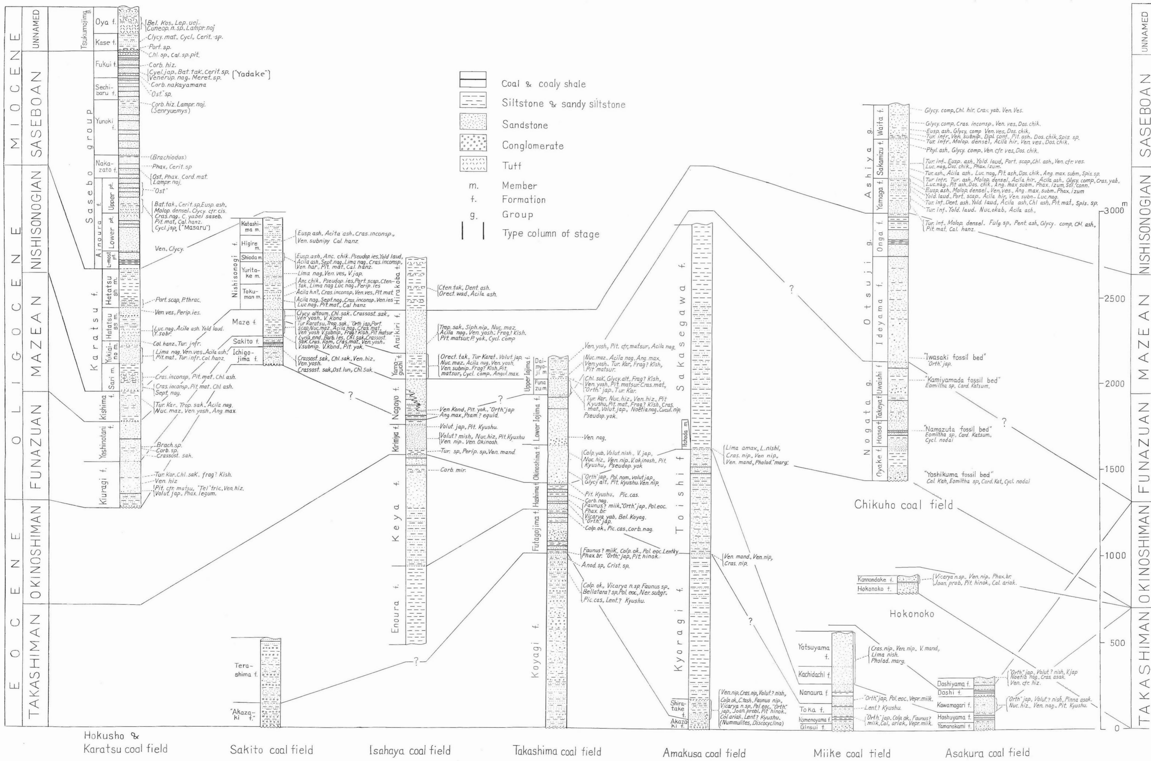
Fig. 2 Columnar sections of the Paleogene and lower Neogene strata in west Japan
