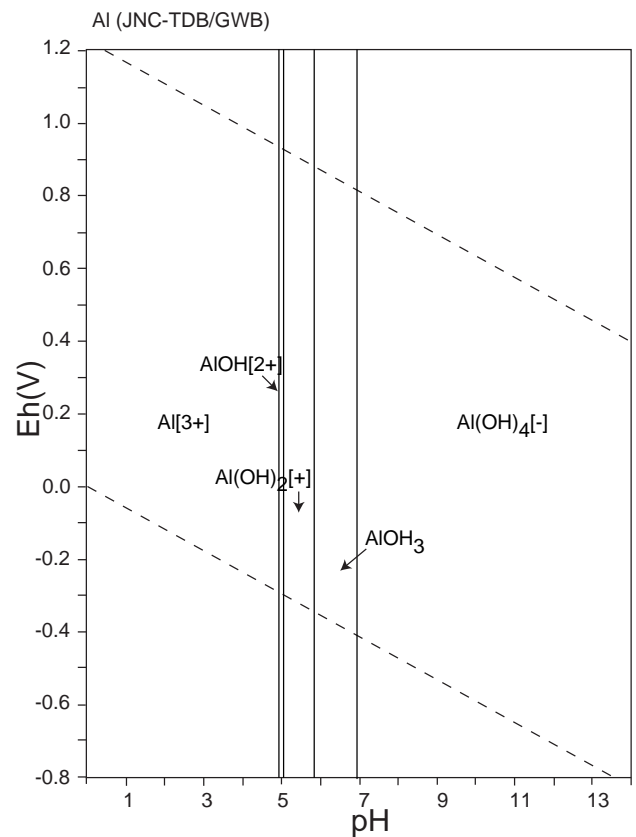
Figure 7: Eh-pH diagrams of the system Al-O-H (1). \Sigma \text{Al} = 10^{-10} , 298.15K, 10^5 Pa.
