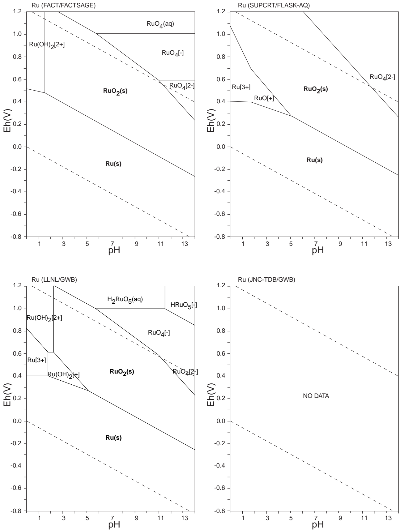
Figure 104: Eh-pH diagrams of the system Ru-O-H (1). \sum \text{Ru} = 10^{-10} , 298.15K, 10^5 Pa.
