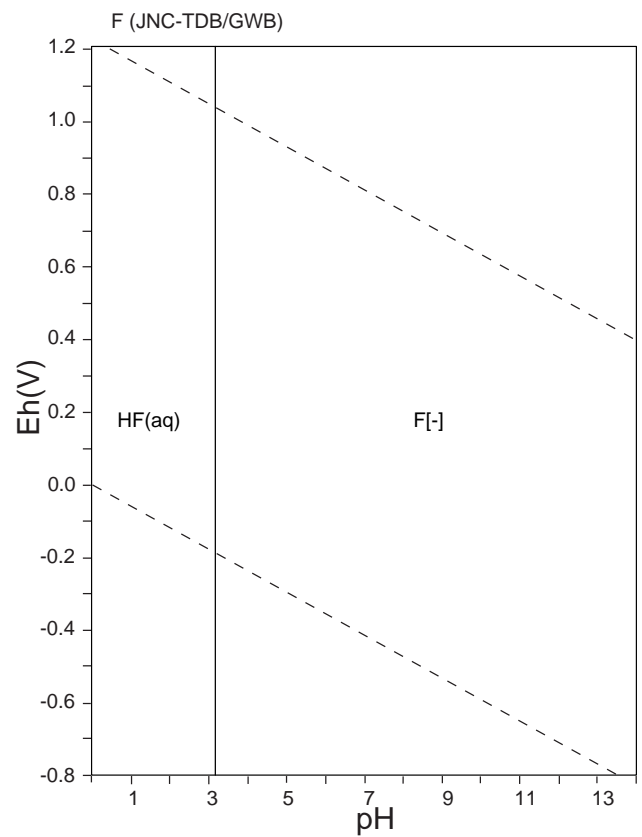
Figure 45: Eh-pH diagrams of the system F-O-H (1). \sum F = 10^{-10} , 298.15K, 10^5 Pa.
