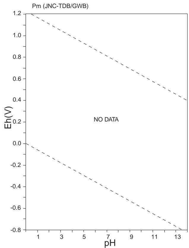
Figure 93: Eh-pH diagrams of the system Pm-O-H. \sum \text{Pm} = 10^{-10} , 298.15K, 10^5 Pa.
