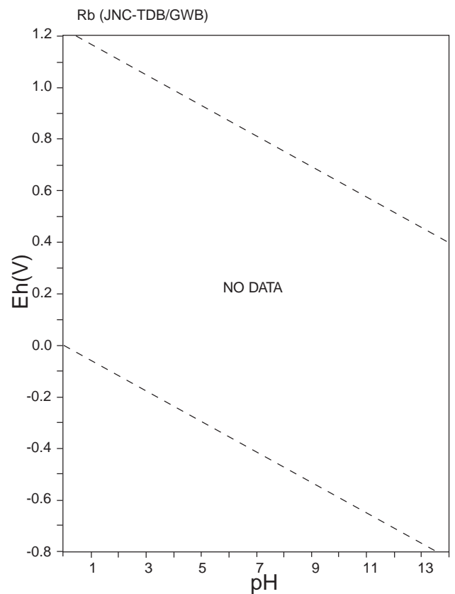
Figure 101: Eh-pH diagrams of the system Rb-O-H. \sum \text{Rb} = 10^{-10} , 298.15K, 10^5 Pa.
