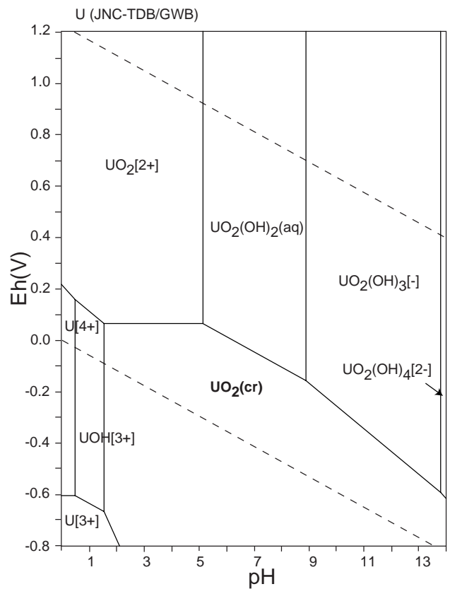
Figure 129: Eh-pH diagrams of the system U-O-H (1). \Sigma U = 10^{-10} , 298.15K, 10^5 Pa.
