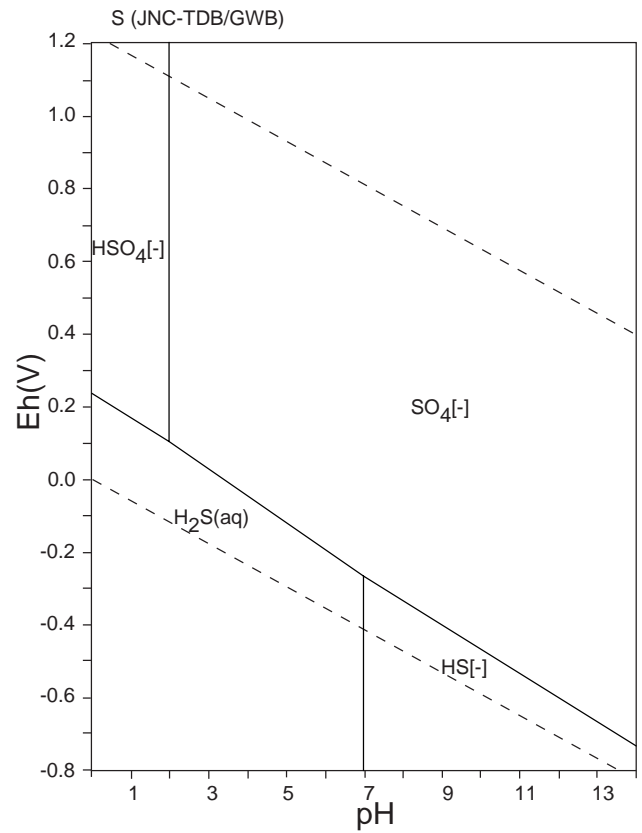
Figure 106: Eh-pH diagrams of the system S-O-H (1). \sum S = 10^{-10} , 298.15K, 10^5 Pa.
