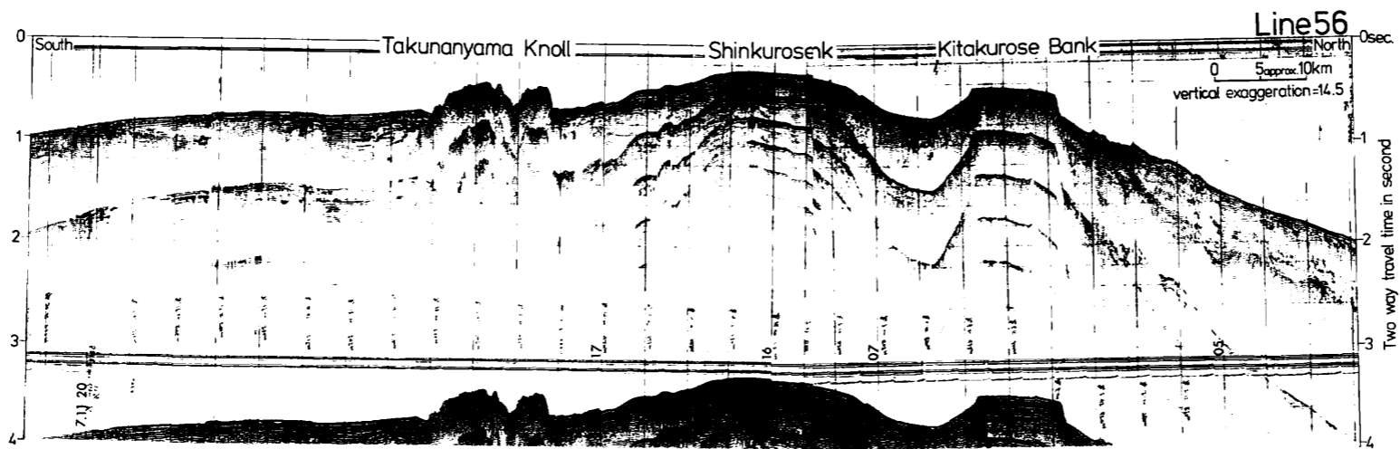
Fig. VI-10 Seismic profiler record of Li 56 by a 120 in 3 air gun with wave shape kit.
