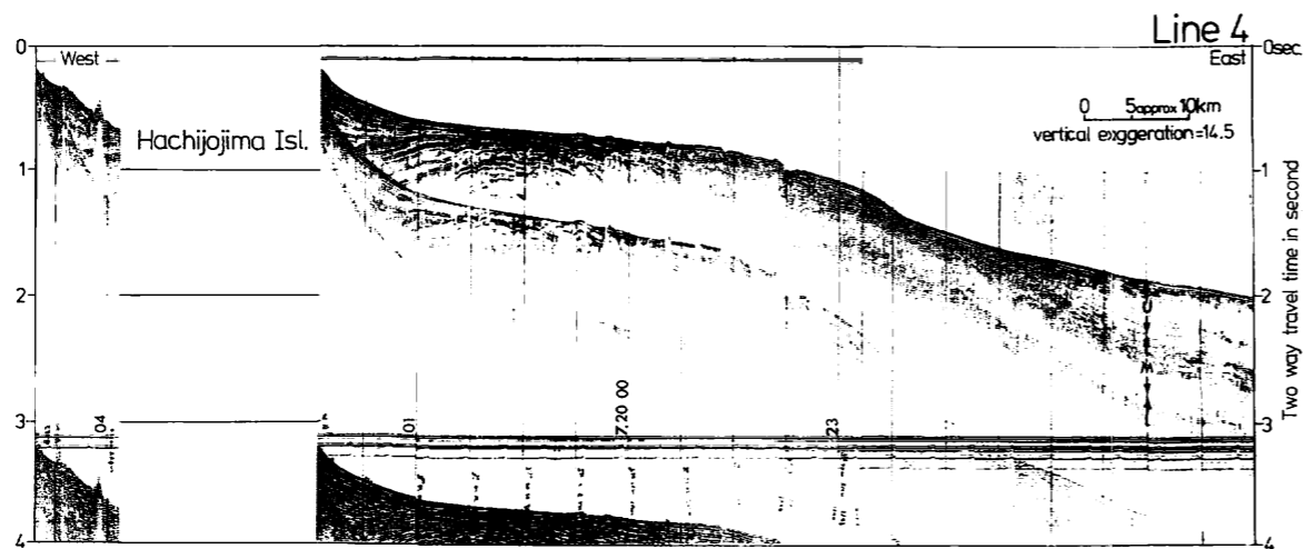
Fig. VI-2 Seismic profiler record of Line 4 by a 120 in 3 air gun with wave shape kit.
