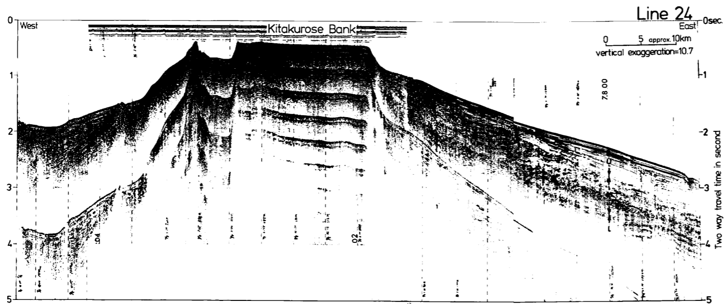
Fig. VI-6 Seismic profiler record of Line 24 by a 150 i 3 air gun.
