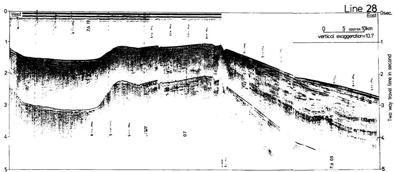
Fig. VI-7 Seismic profiler record of Line 28 by a 150 in 3 air gun.
