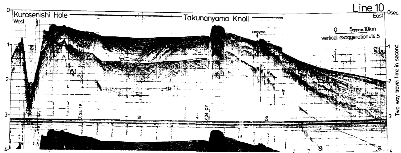
Fig. VI-4 Seismic profiler record of Line 10 by a 120 in 3 air gun with wave shape kit.
