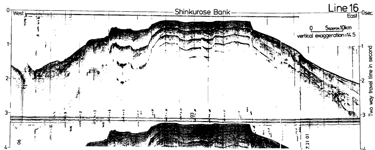
Fig. VI-5 Seismic profiler record of Line 16 by a 120 in 3 air gun with wave shape kit.
