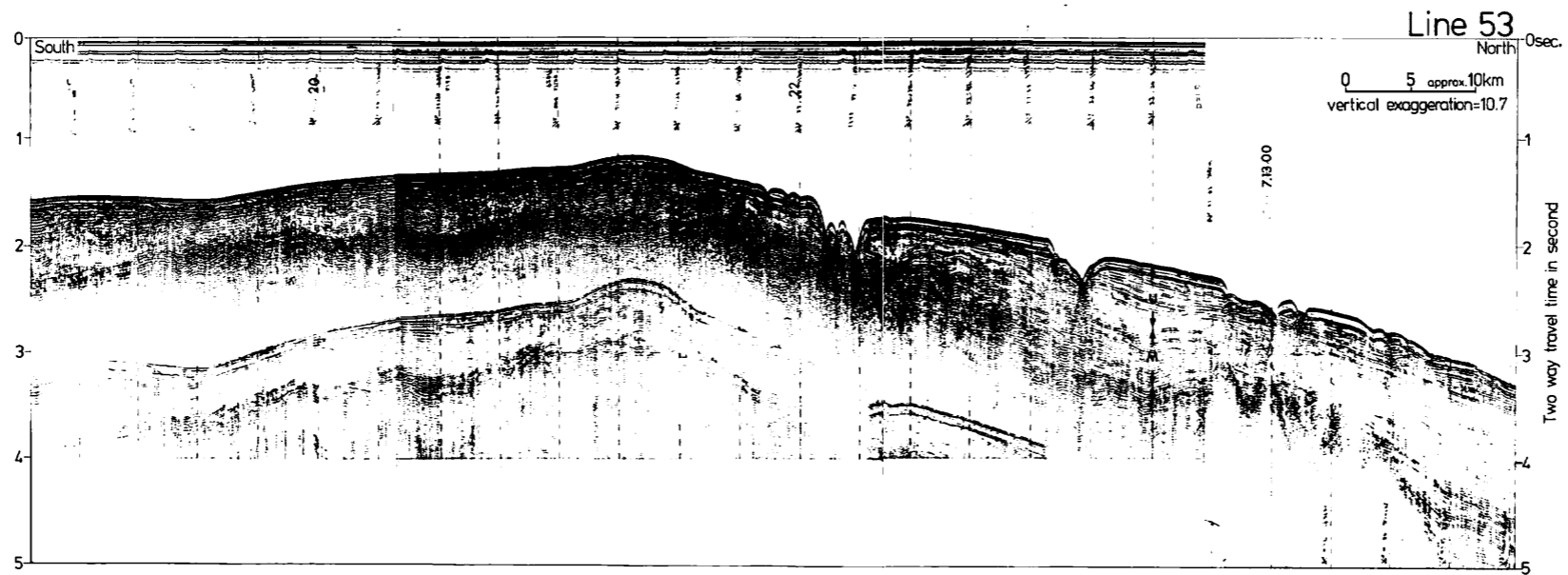
Fig. VI-9 Seismic profiler record of Line 53 by a 150 in 3 air gun.
