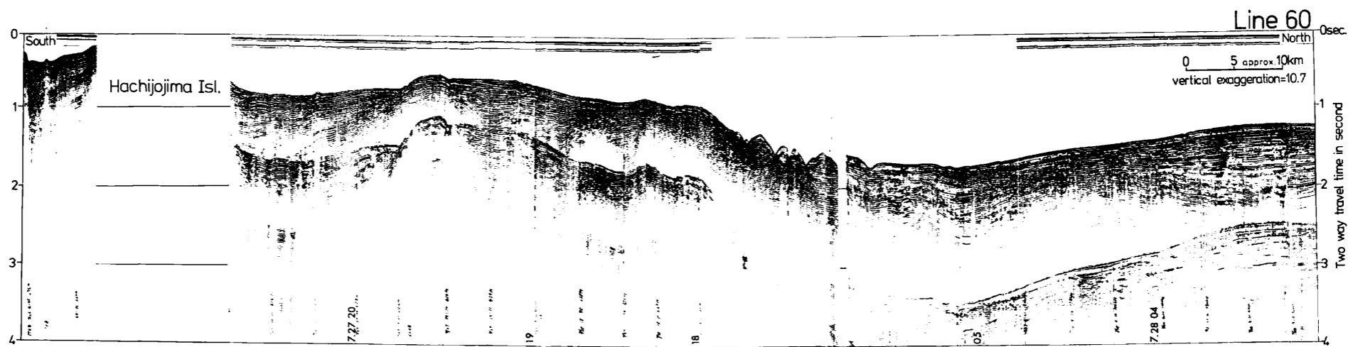
Fig. VI-11 Seismic profiler recrd of Line 60 by a 150 in 3 air gun.
