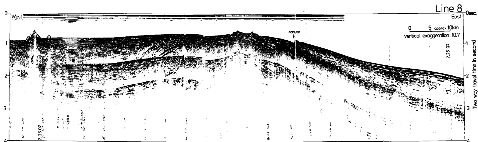
Fig. VI-3 Seismic profiler record of Line 8 by a 150 in 3 air gun.
