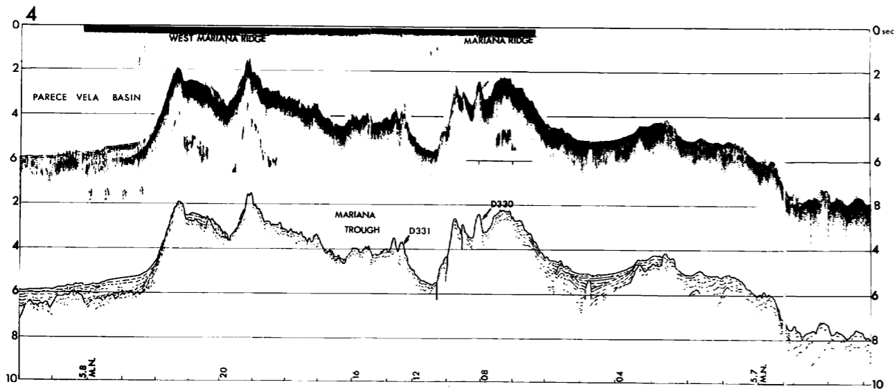
Fig VI-1-a Seismic profiles with interpretative line drawings.
