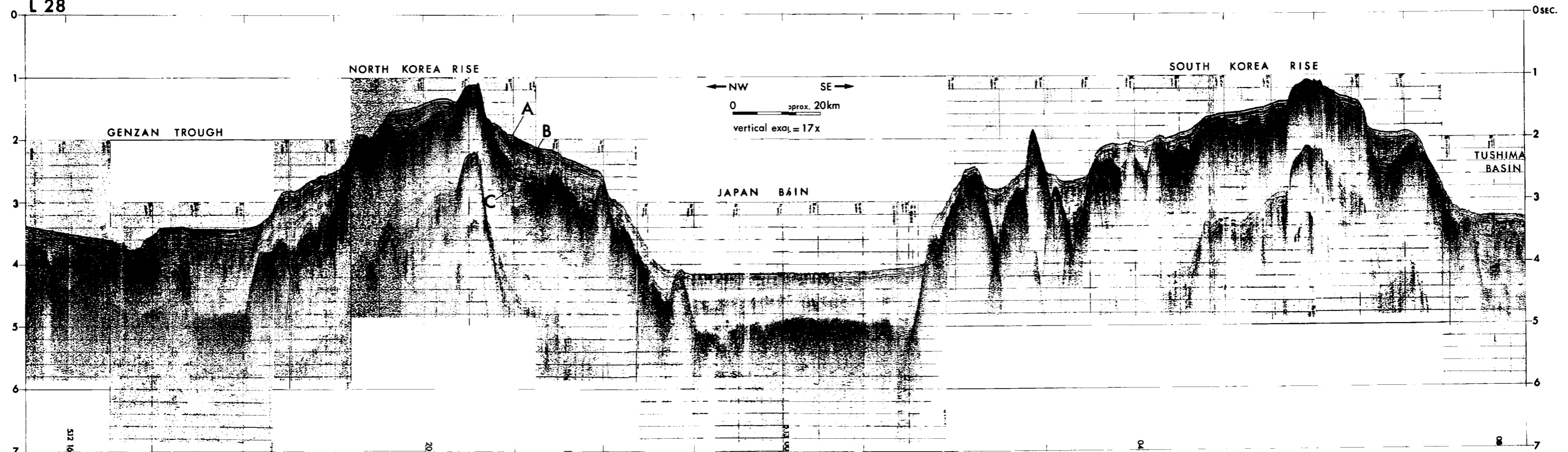
Fig. VI-4 Seismic profiler record across the Korea Continental Borderland of Line 28 in Fig. I-1. Vertical scale presented in two way travel time. A: the upper sedimentary unit, B: the middle sedimentary unit and C: the lower sedimentary unit on the rises.
