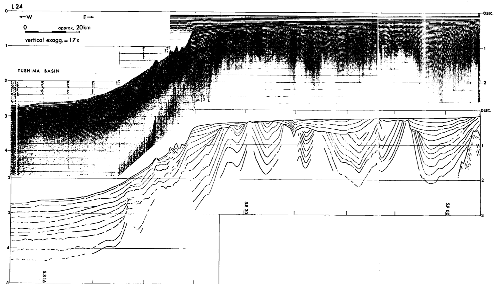
Fig. VI-2 Seismic profiler record with interpretation of Line 24 in Fig. I-1. Vertical scale is presented in seconds of two way travel time.
