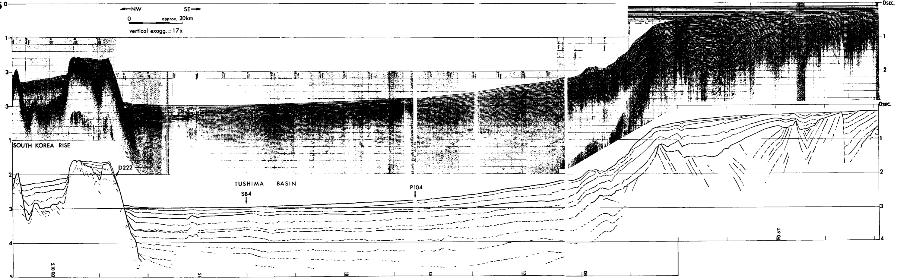
Fig. VI-3 Seismic profiler record with interpretation of Line 25 in Fig. I-1. Vertical scale is presented in seconds of two way travel time.
