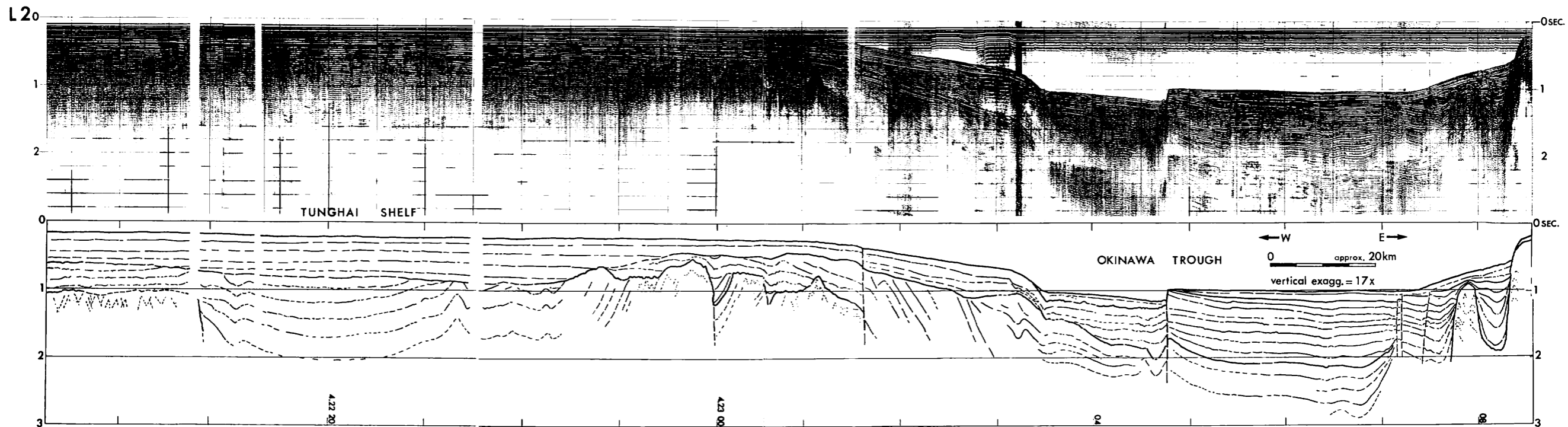
Fig. VI-1 Seismic profiler record with interpretation of Line 2 in Fig. I-1. Vertical scale is presented in seconds of two way travel time.
