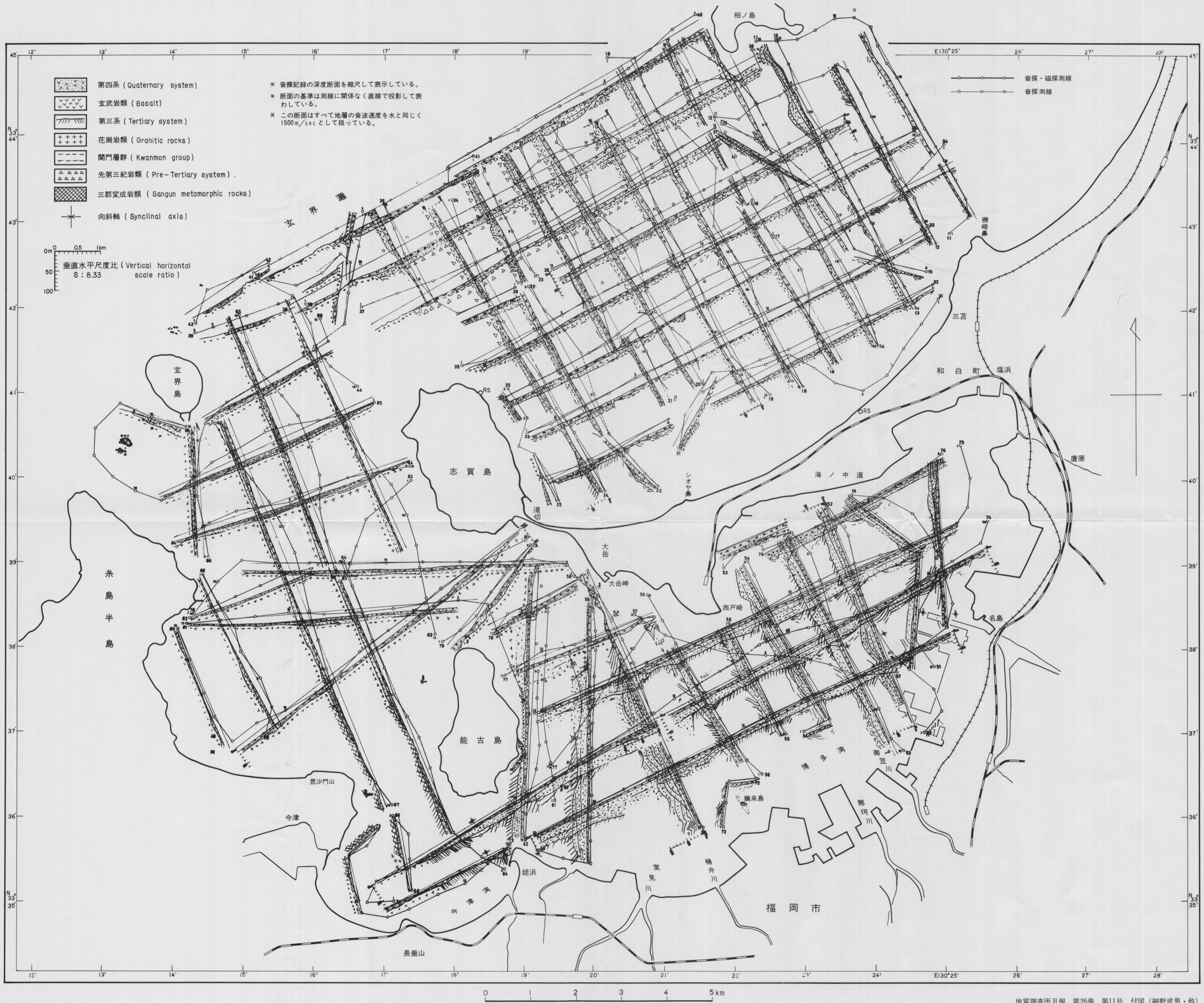
第6図 志賀島周辺海域音波探査解析断面図 Fig. 6 Interpreted Cross Sections of Sparker's Reflection Profile around Shikanoshima Island
