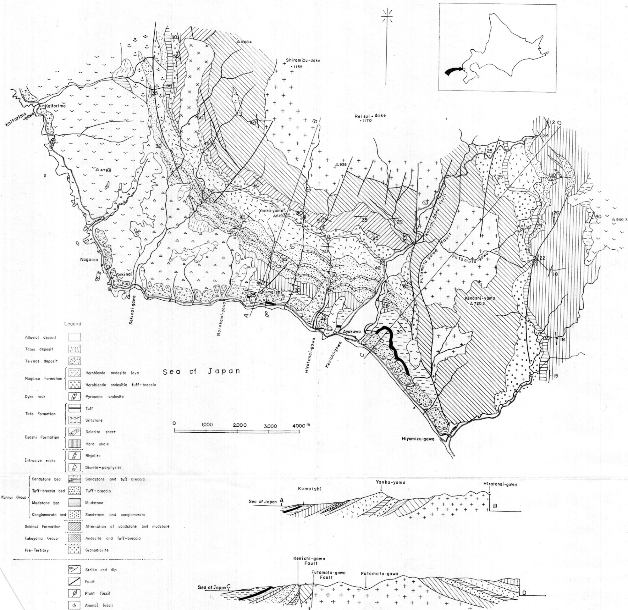
Fig. 1 Geological map of Kumaishi area
